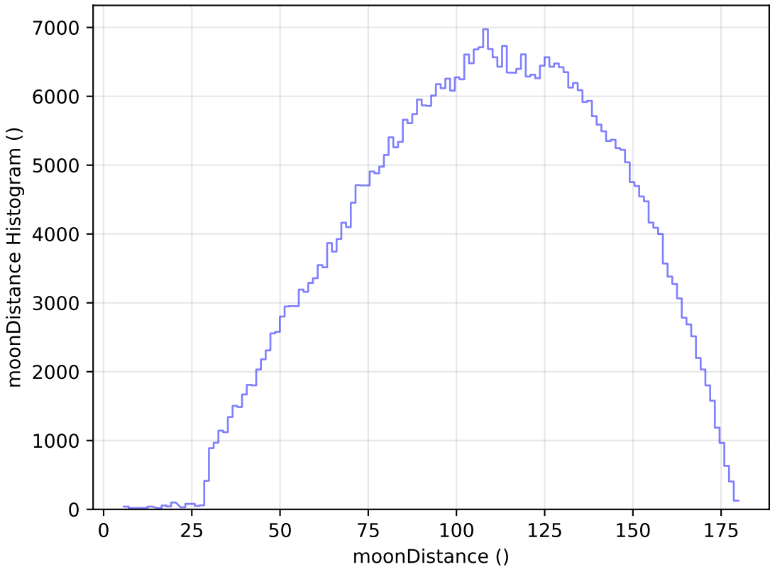
too_ignore_5_1v3.4_10yrs All sky r band: moonDistance Histogram
