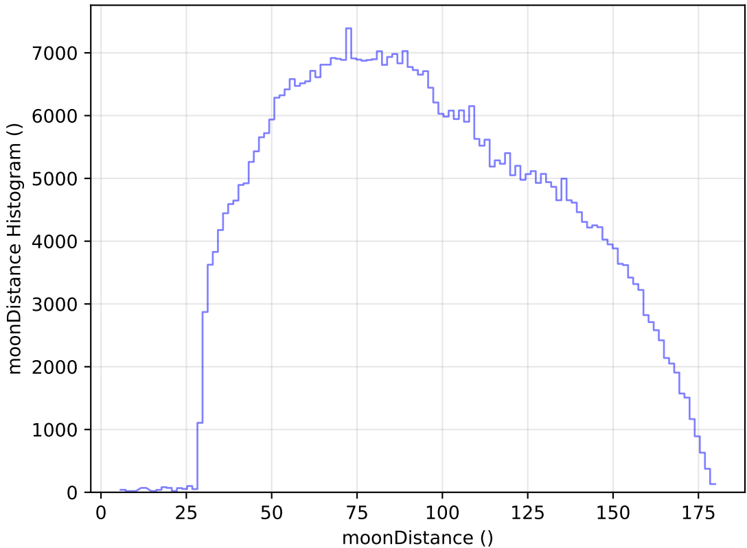
too_ignore_5_1v3.4_10yrs All sky i band: moonDistance Histogram
