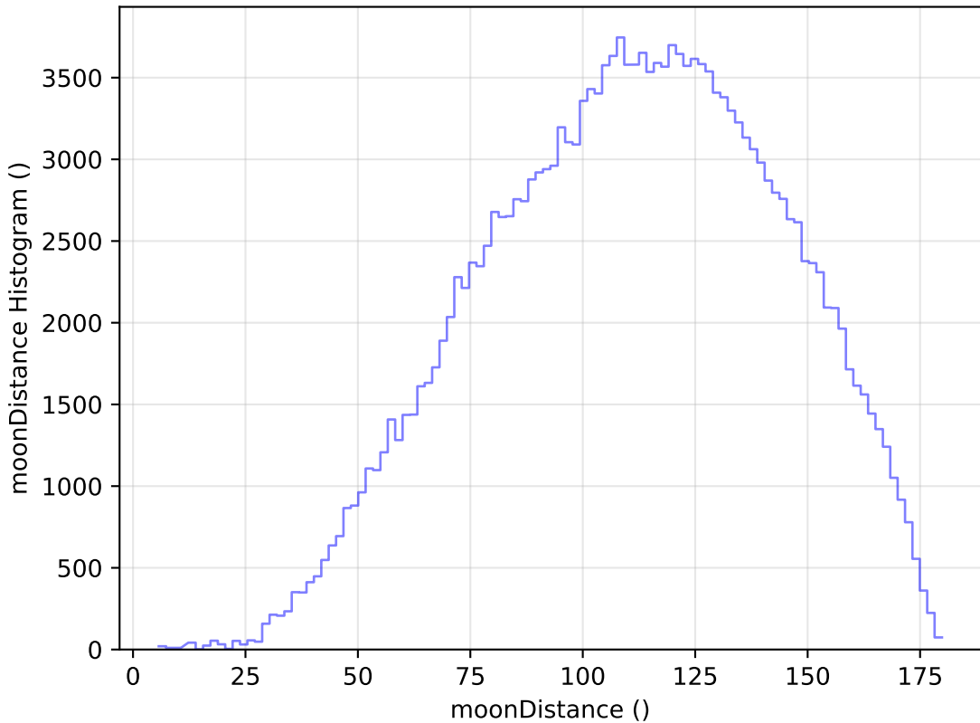
too_ignore_5_1v3.4_10yrs All sky g band: moonDistance Histogram
