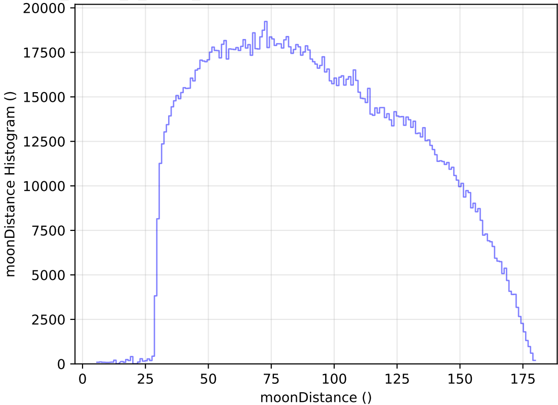
too_ignore_5_1v3.4_10yrs All sky all bands: moonDistance Histogram
