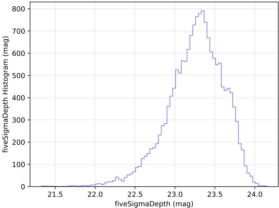
too_ignore_5_1v3.4_10yrs Yr 1 u band: fiveSigmaDepth Histogram
