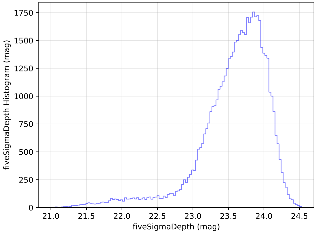
too_ignore_5_1v3.4_10yrs Yr 1 i band: fiveSigmaDepth Histogram
