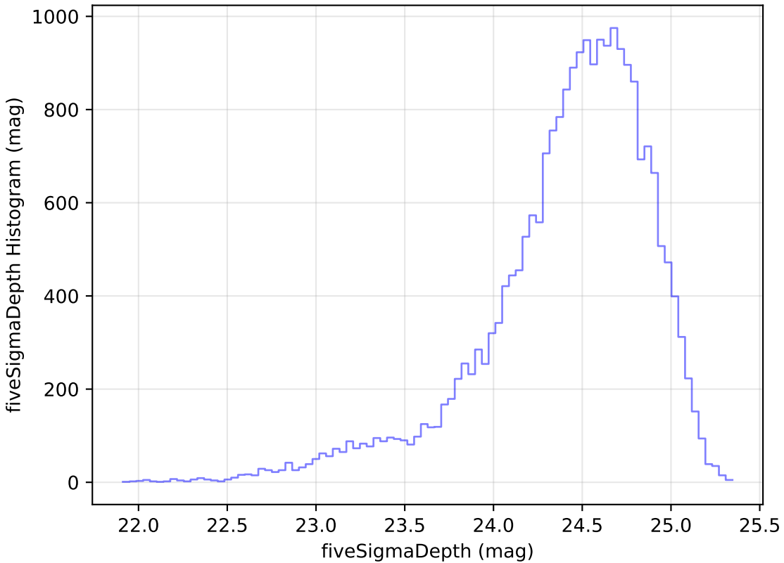
too_ignore_5_1v3.4_10yrs Yr 1 g band: fiveSigmaDepth Histogram
