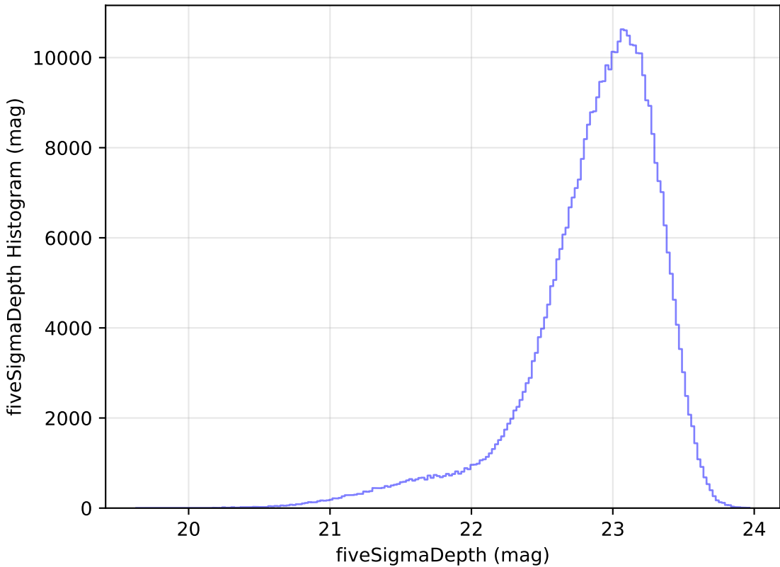
too_ignore_5_1v3.4_10yrs WFD z band: fiveSigmaDepth Histogram
