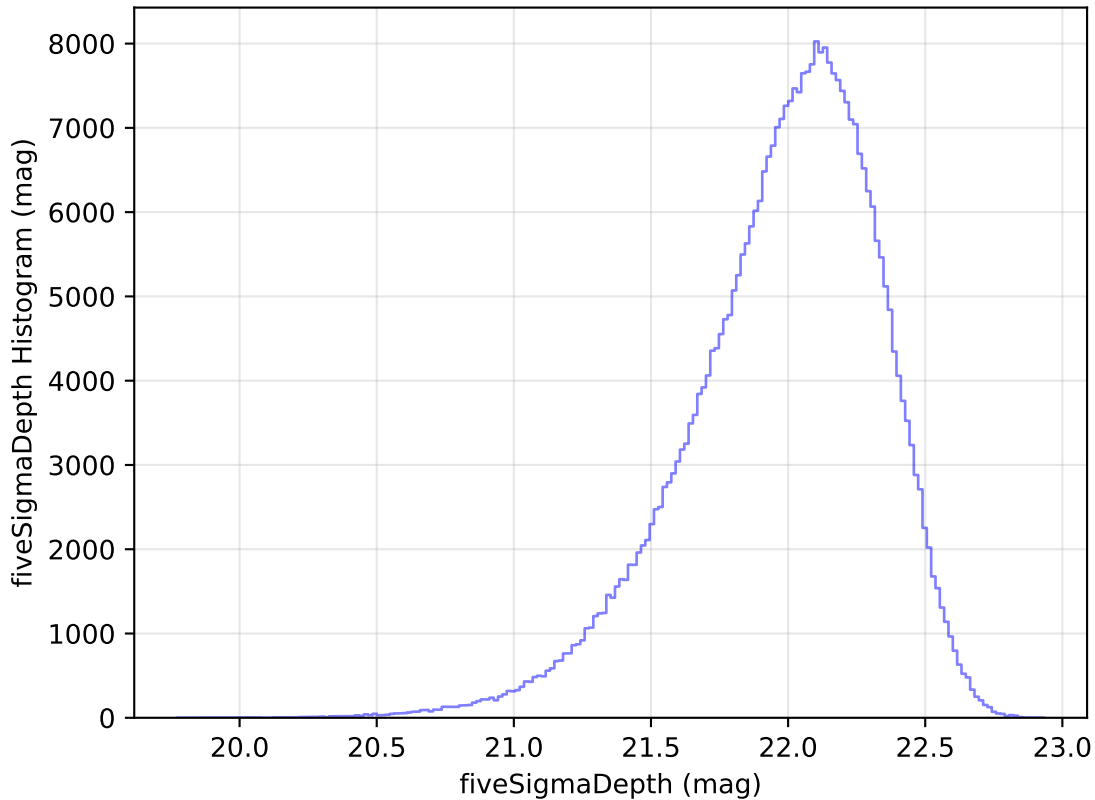
too_ignore_5_1v3.4_10yrs WFD y band: fiveSigmaDepth Histogram
