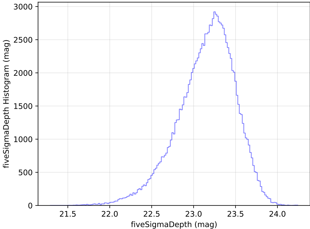
too_ignore_5_1v3.4_10yrs WFD u band: fiveSigmaDepth Histogram
