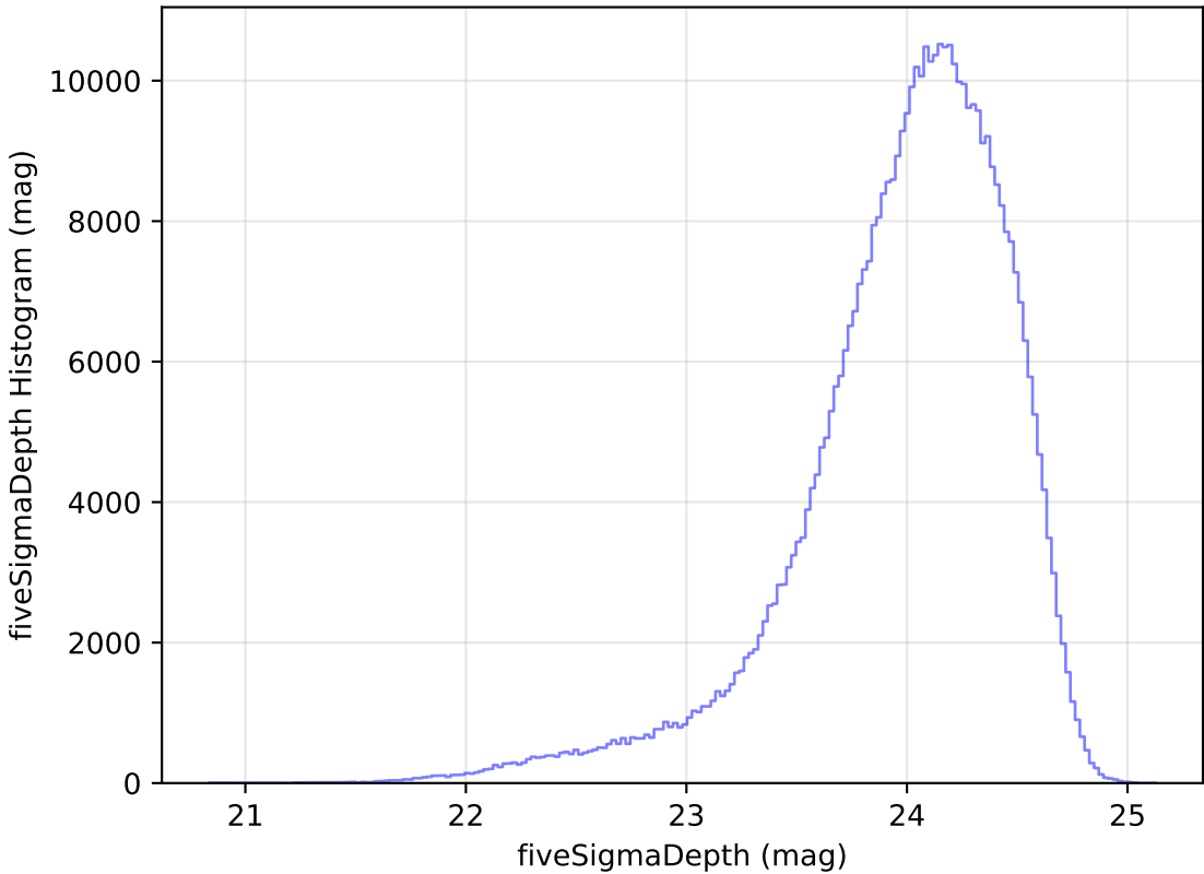
too_ignore_5_1v3.4_10yrs WFD r band: fiveSigmaDepth Histogram
