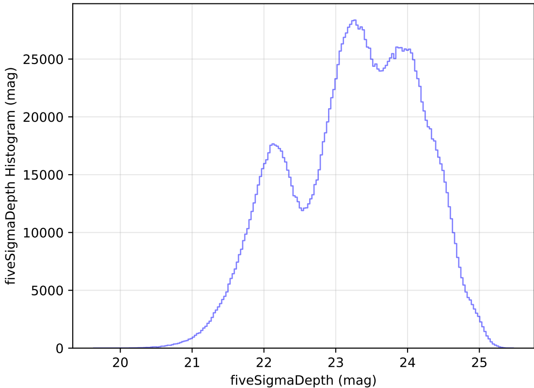
too_ignore_5_1v3.4_10yrs WFD all bands: fiveSigmaDepth Histogram
