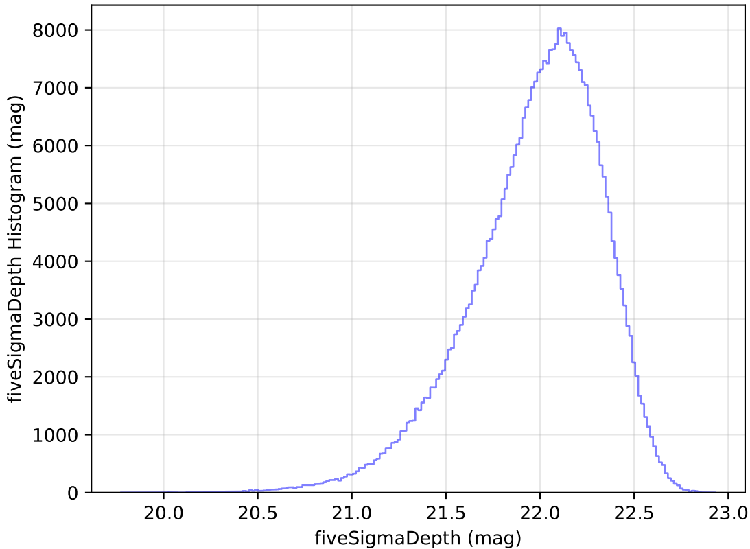
too_ignore_5_1v3.4_10yrs All sky y band: fiveSigmaDepth Histogram
