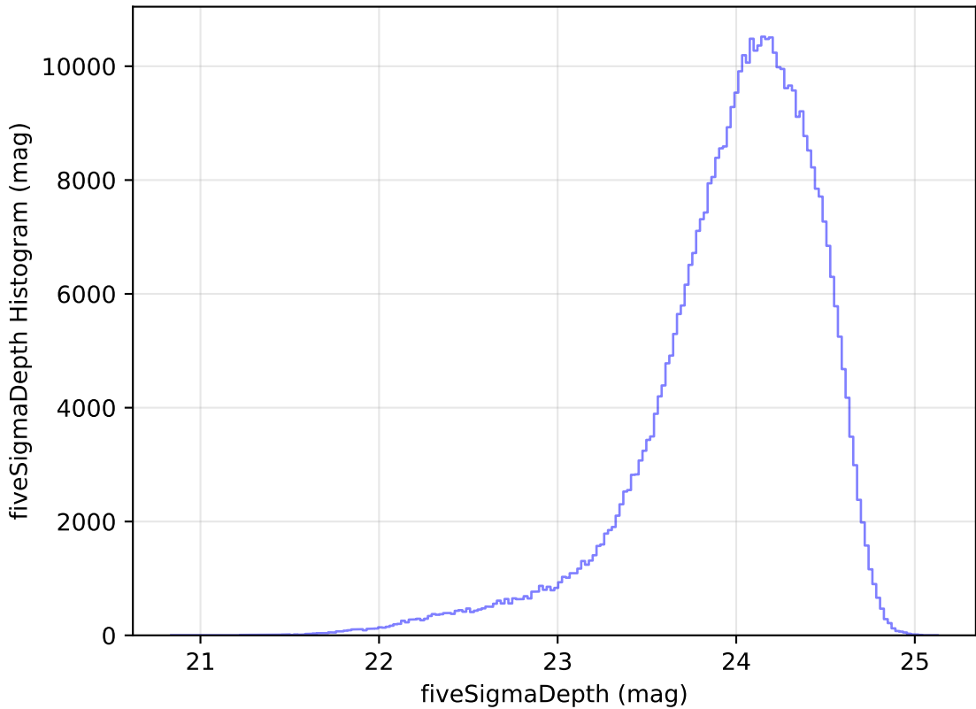
too_ignore_5_1v3.4_10yrs All sky r band: fiveSigmaDepth Histogram
