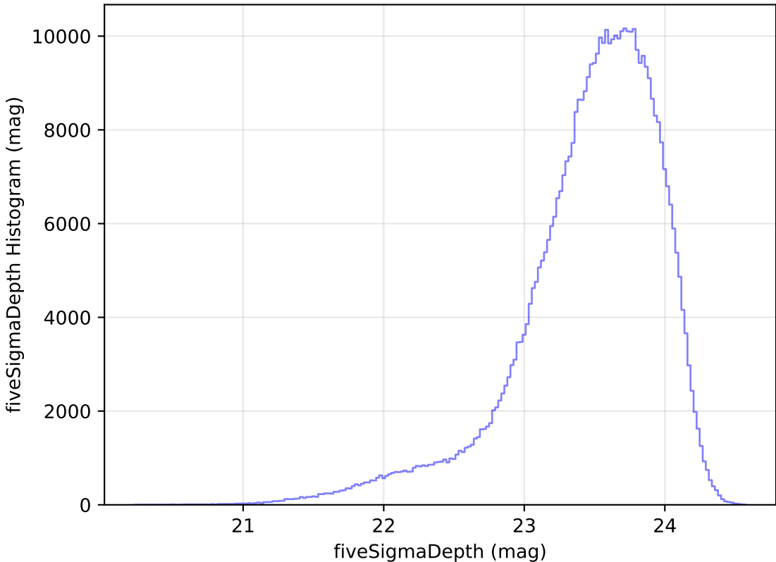
too_ignore_5_1v3.4_10yrs All sky i band: fiveSigmaDepth Histogram
