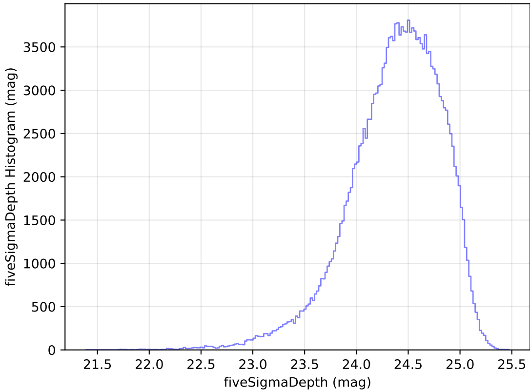
too_ignore_5_1v3.4_10yrs All sky g band: fiveSigmaDepth Histogram
