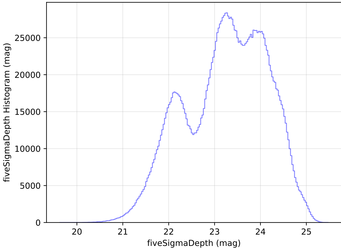
too_ignore_5_1v3.4_10yrs All sky all bands: fiveSigmaDepth Histogram
