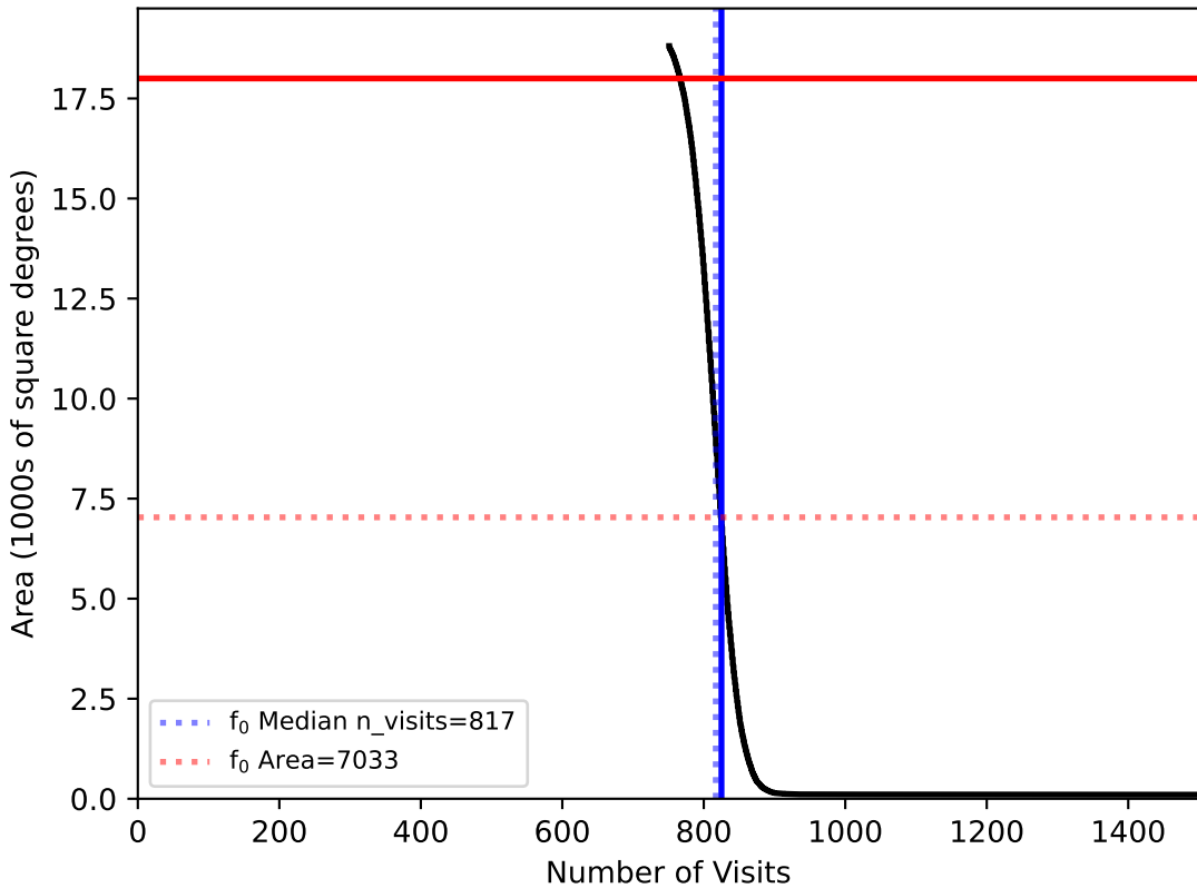
too_ignore_5_1v3.4_10yrs WFD: fO
