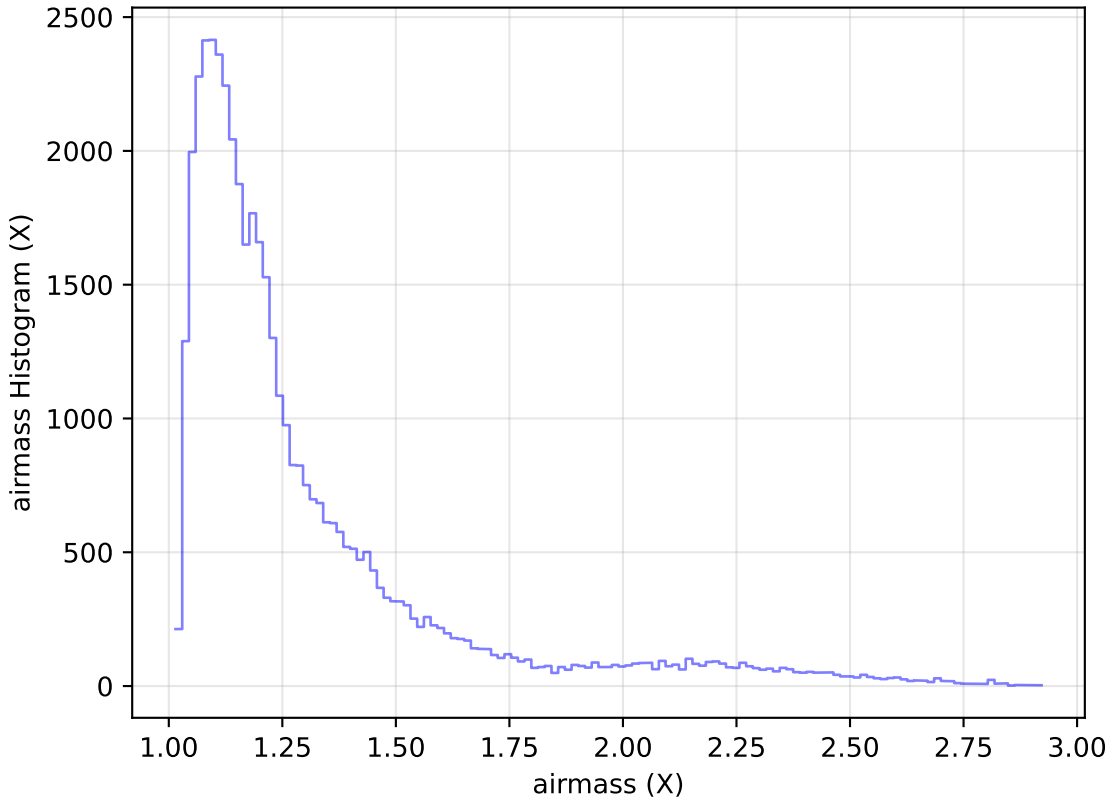
too_ignore_5_1v3.4_10yrs Yr 1 z band: airmass Histogram
