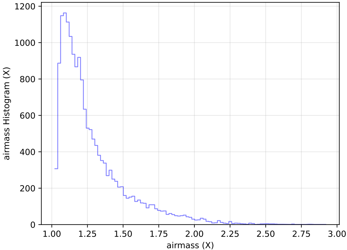
too_ignore_5_1v3.4_10yrs Yr 1 u band: airmass Histogram
