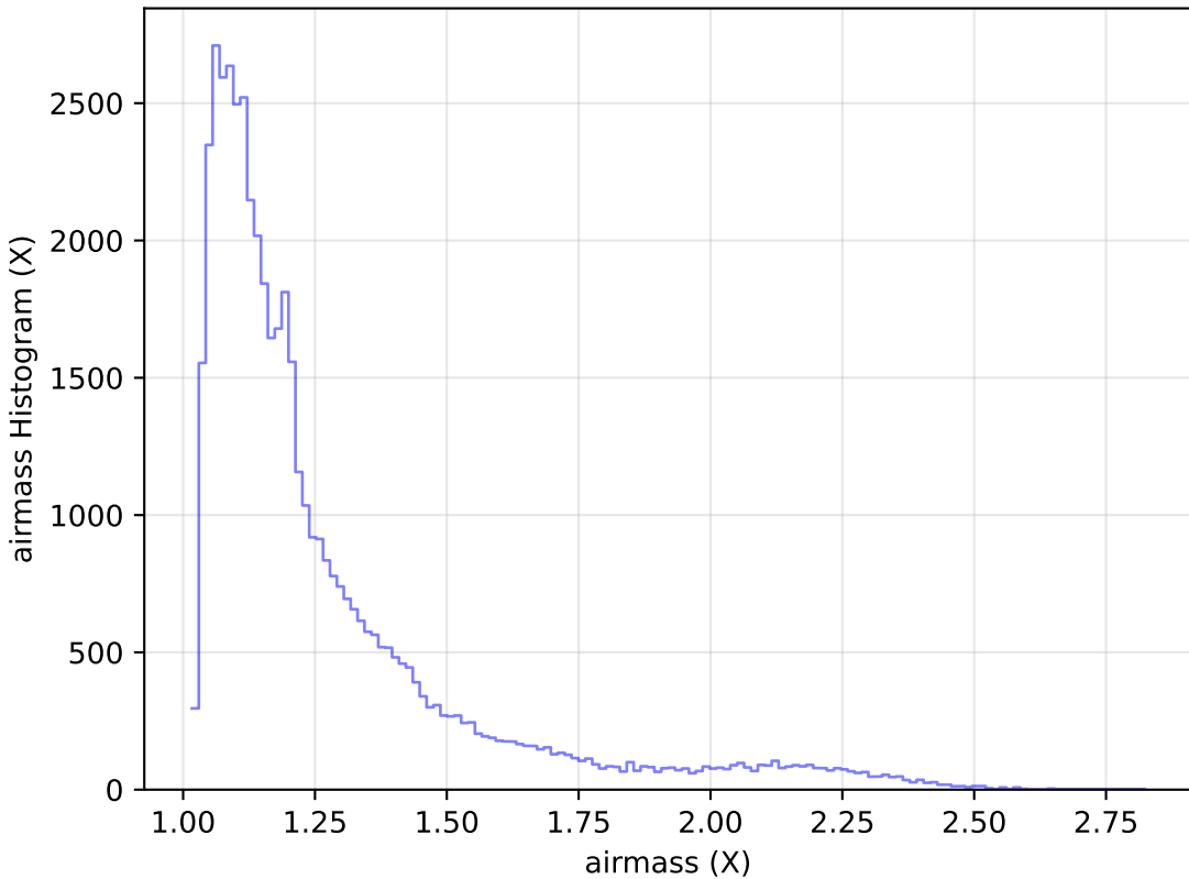
too_ignore_5_1v3.4_10yrs Yr 1 r band: airmass Histogram
