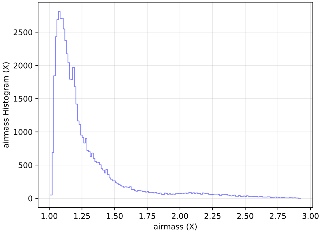
too_ignore_5_1v3.4_10yrs Yr 1 i band: airmass Histogram
