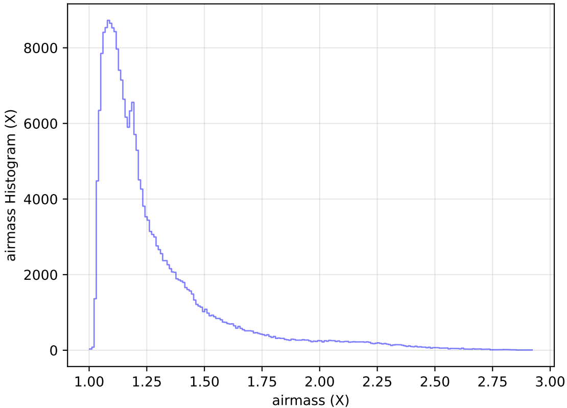
too_ignore_5_1v3.4_10yrs Yr 1 all bands: airmass Histogram
