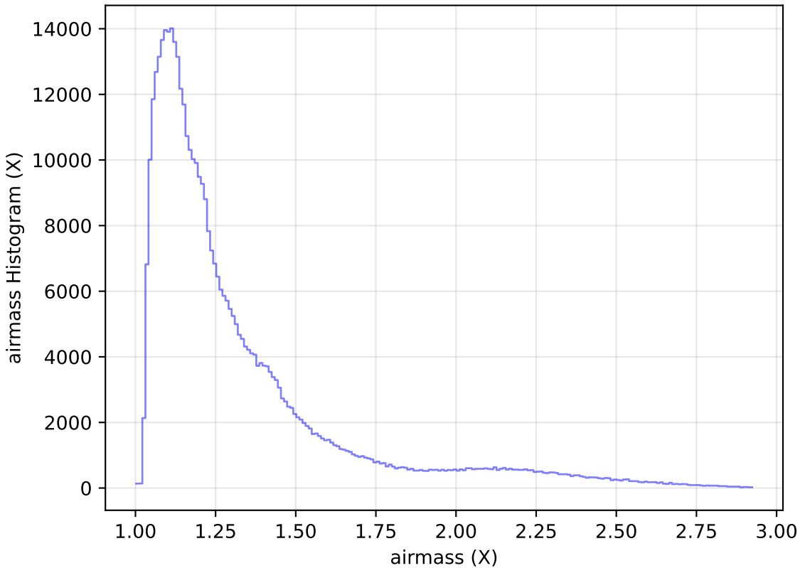
too_ignore_5_1v3.4_10yrs WFD z band: airmass Histogram
