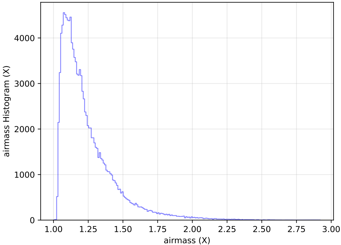
too_ignore_5_1v3.4_10yrs WFD u band: airmass Histogram
