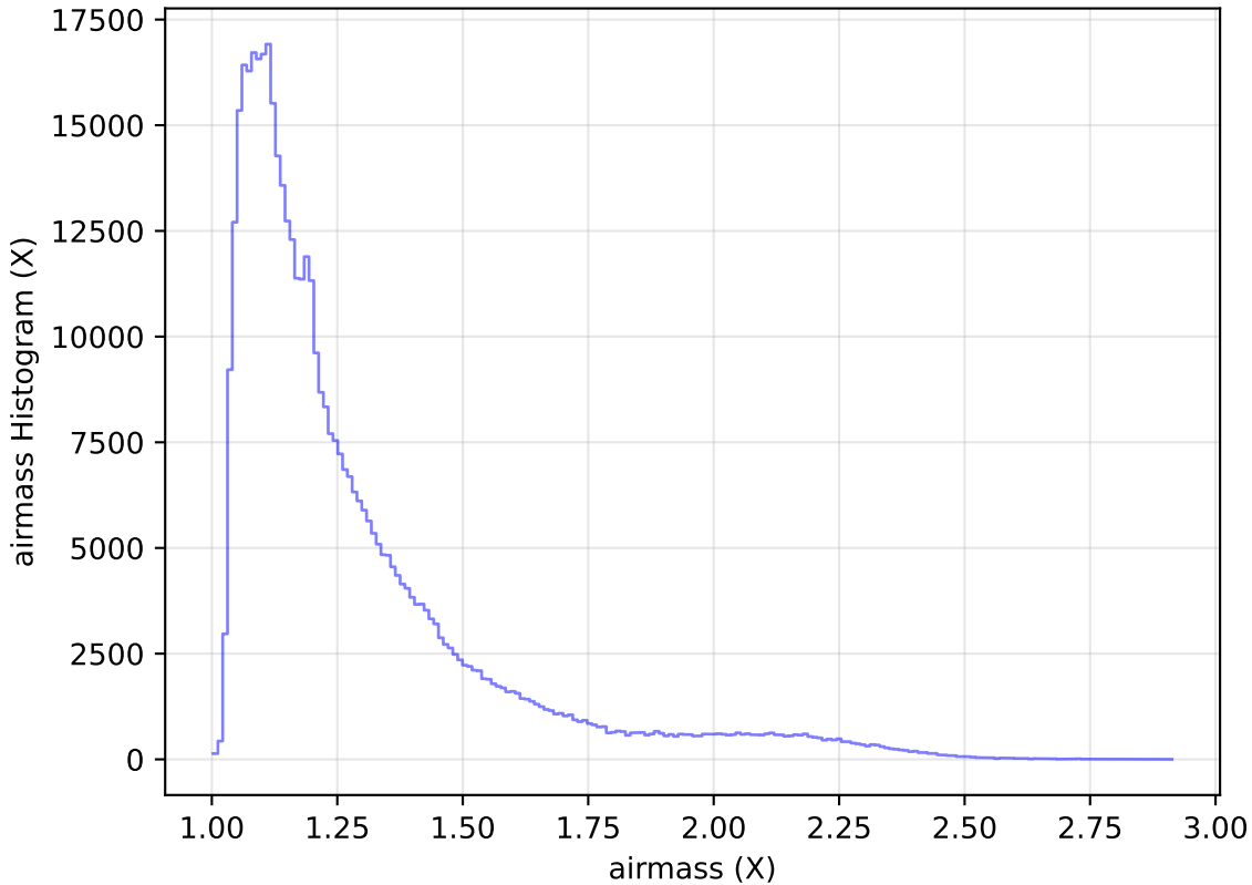
too_ignore_5_1v3.4_10yrs WFD r band: airmass Histogram
