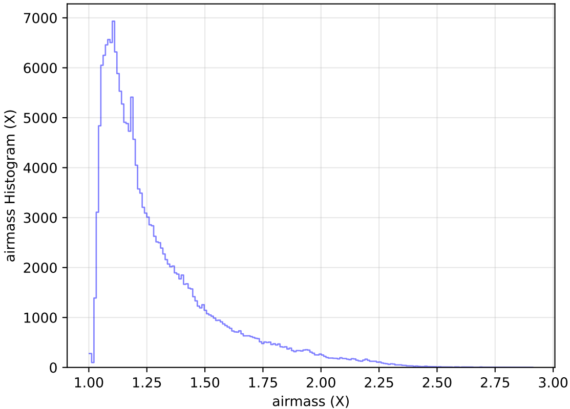
too_ignore_5_1v3.4_10yrs WFD g band: airmass Histogram
