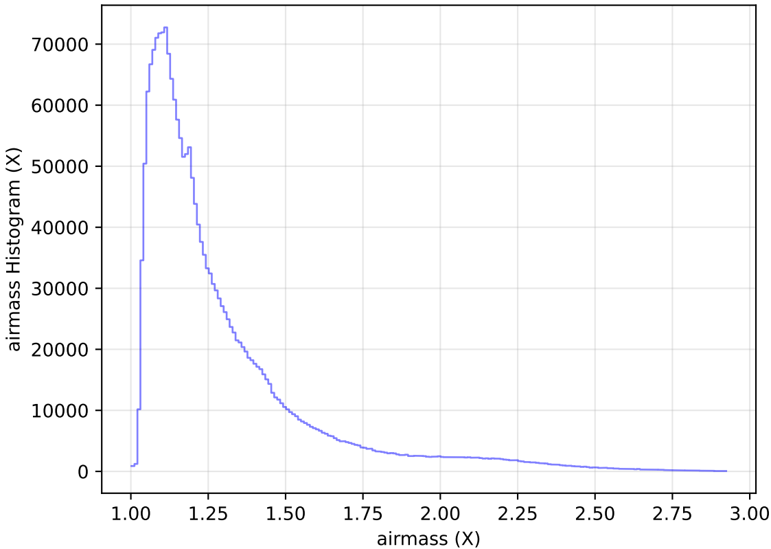
too_ignore_5_1v3.4_10yrs WFD all bands: airmass Histogram
