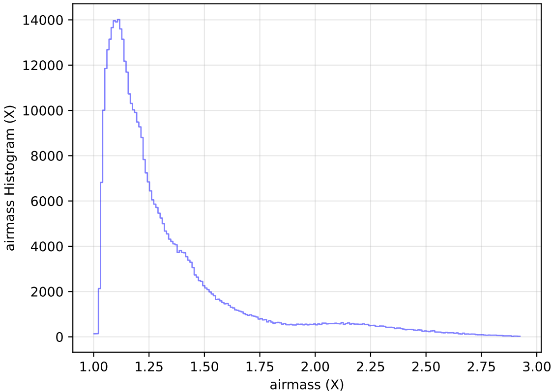
too_ignore_5_1v3.4_10yrs All sky z band: airmass Histogram
