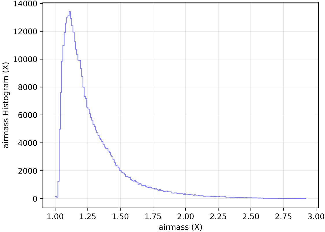
too_ignore_5_1v3.4_10yrs All sky y band: airmass Histogram
