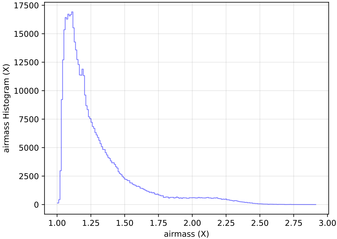
too_ignore_5_1v3.4_10yrs All sky r band: airmass Histogram
