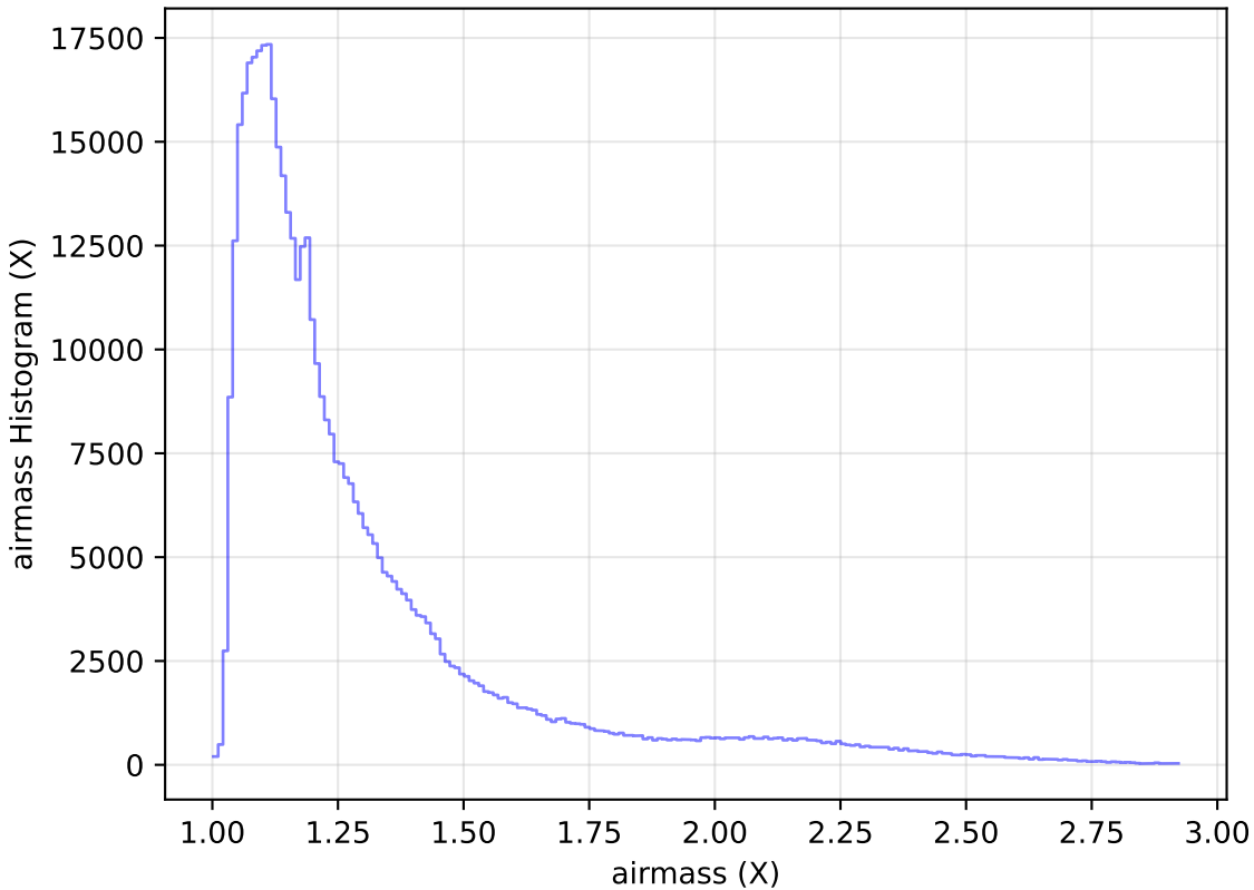
too_ignore_5_1v3.4_10yrs All sky i band: airmass Histogram
