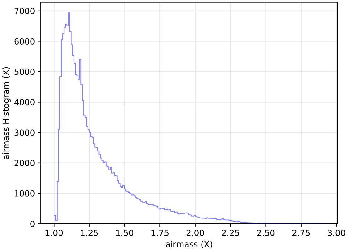
too_ignore_5_1v3.4_10yrs All sky g band: airmass Histogram
