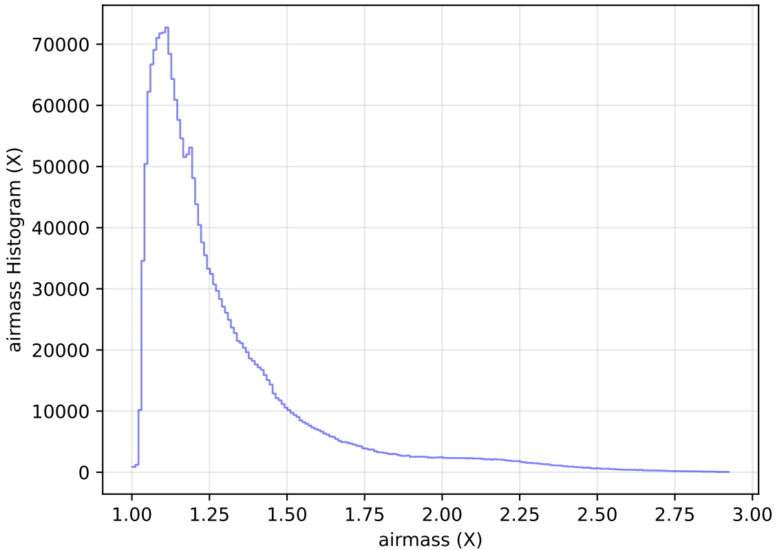
too_ignore_5_1v3.4_10yrs All sky all bands: airmass Histogram
