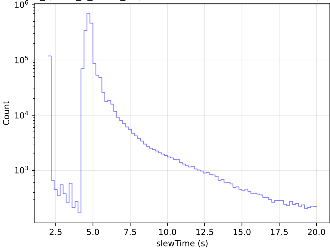
too_ignore_5_1v3.4_10yrs All visits: Zoom Slew Time Histogram
