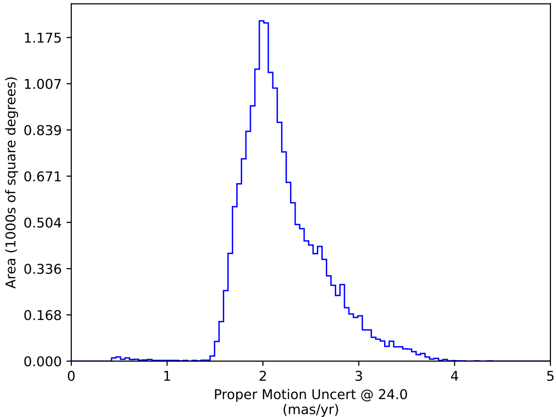
too_ignore_5_1v3.4_10yrs WFD: Proper Motion Uncert @ 24.0
