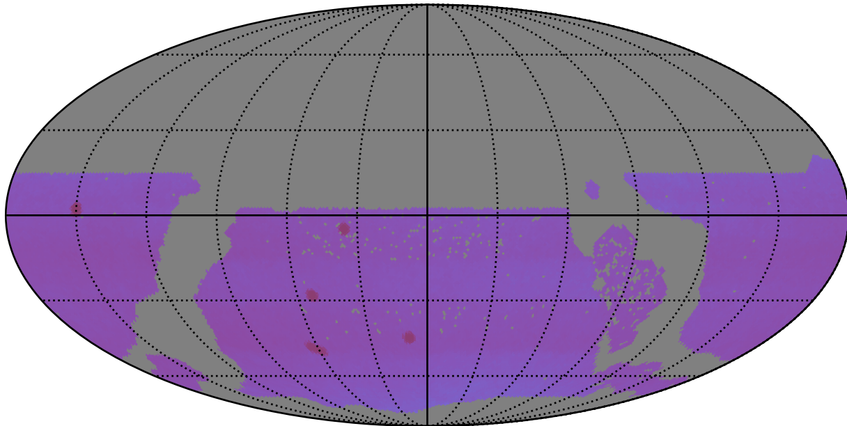
too_ignore_5_1v3.4_10yrs WFD: Proper Motion Uncert @ 20.5
