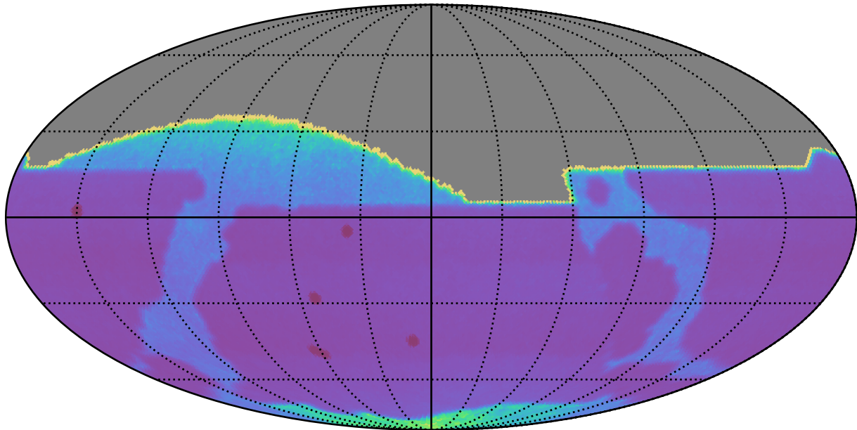
too_ignore_5_1v3.4_10yrs All sky: Proper Motion Uncert @ 20.5
