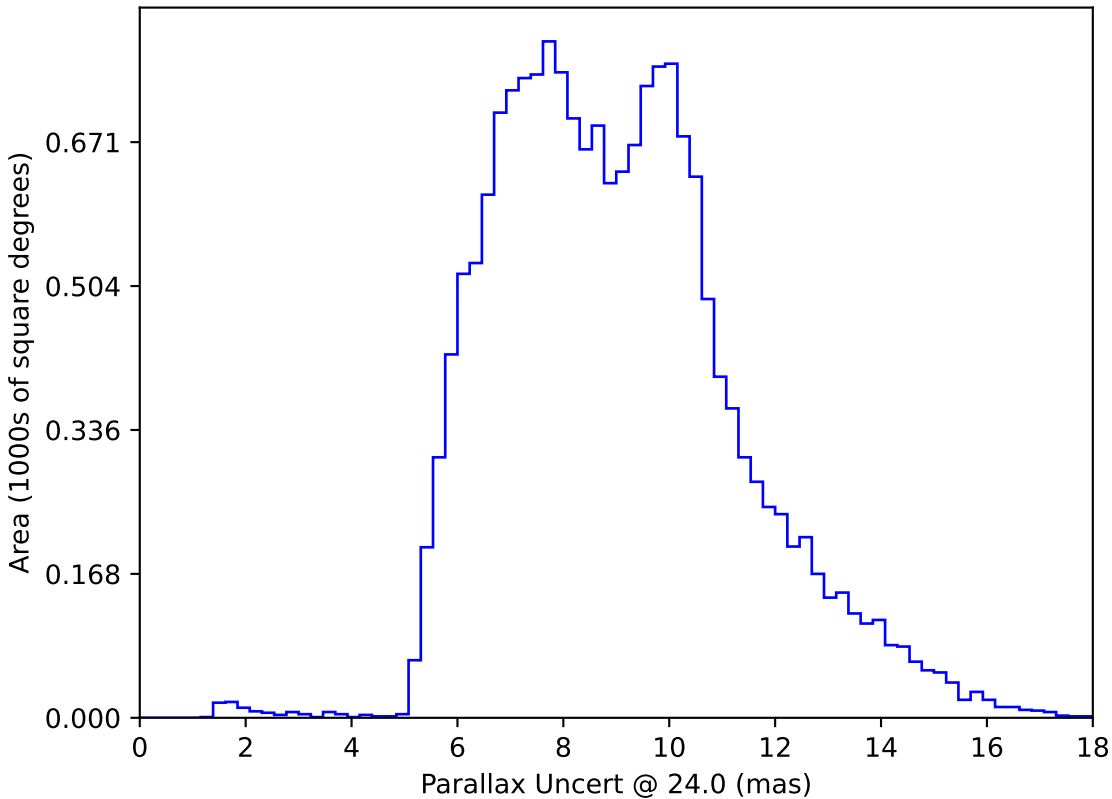
too_ignore_5_1v3.4_10yrs WFD: Parallax Uncert @ 24.0
