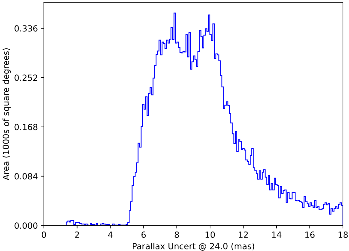
too_ignore_5_1v3.4_10yrs All sky: Parallax Uncert @ 24.0
