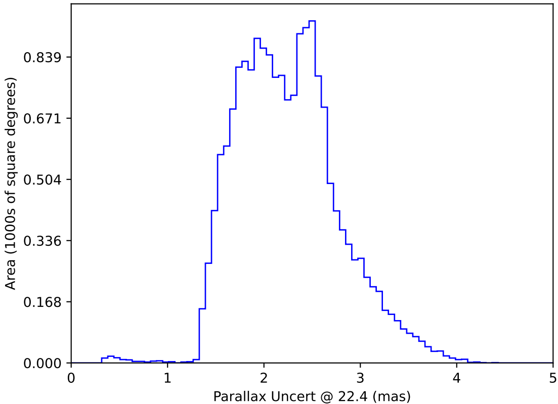
too_ignore_5_1v3.4_10yrs WFD: Parallax Uncert @ 22.4
