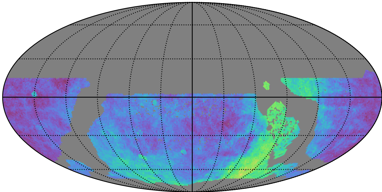
too_ignore_5_1v3.4_10yrs WFD: Parallax Coverage @ 24.0
