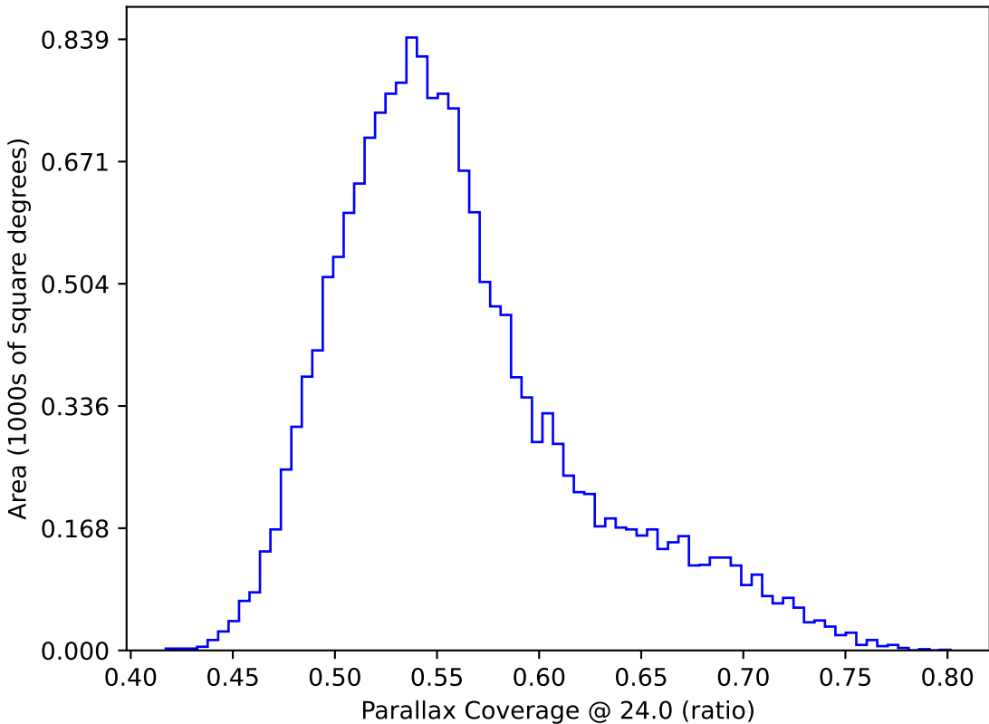
too_ignore_5_1v3.4_10yrs WFD: Parallax Coverage @ 24.0
