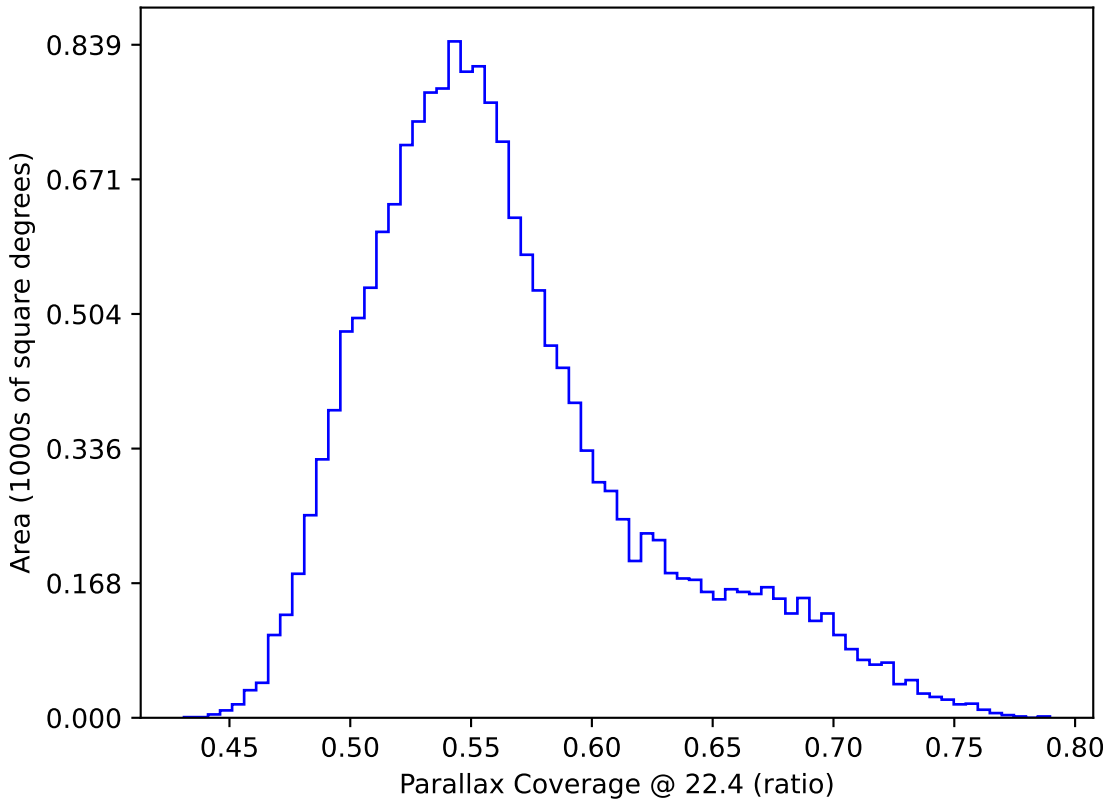
too_ignore_5_1v3.4_10yrs WFD: Parallax Coverage @ 22.4
