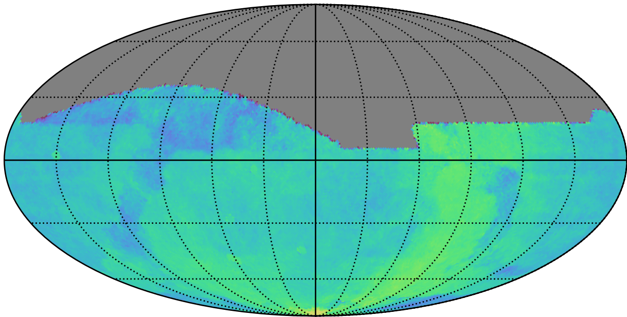
too_ignore_5_1v3.4_10yrs All sky: Parallax Coverage @ 22.4
