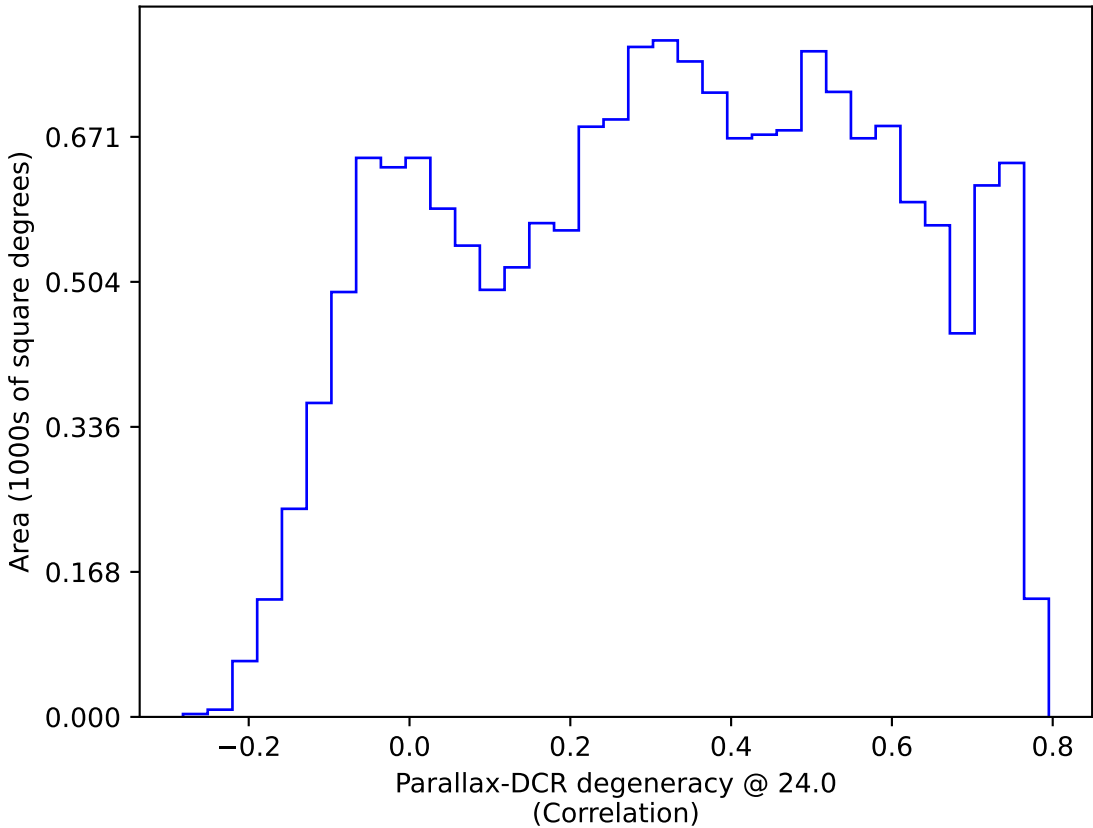
too_ignore_5_1v3.4_10yrs WFD: Parallax-DCR degeneracy @ 24.0
