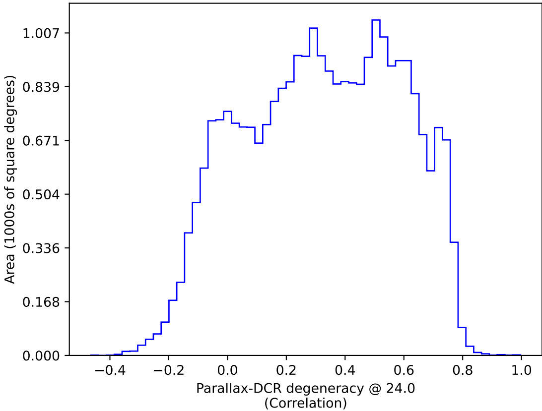
too_ignore_5_1v3.4_10yrs All sky: Parallax-DCR degeneracy @ 24.0
