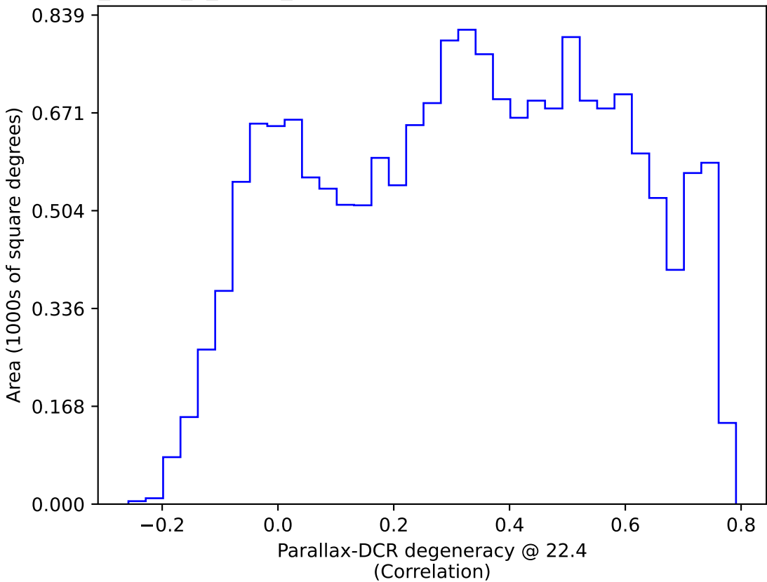
too_ignore_5_1v3.4_10yrs WFD: Parallax-DCR degeneracy @ 22.4
