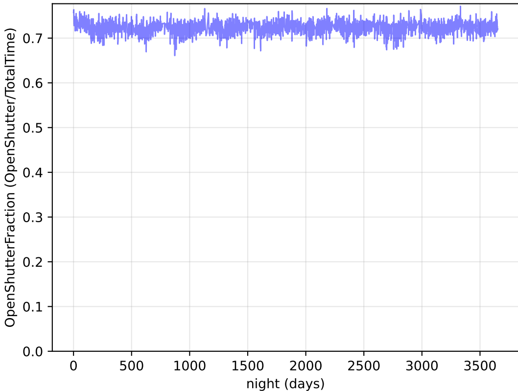
too_ignore_5_1v3.4_10yrs Per night: OpenShutterFraction
