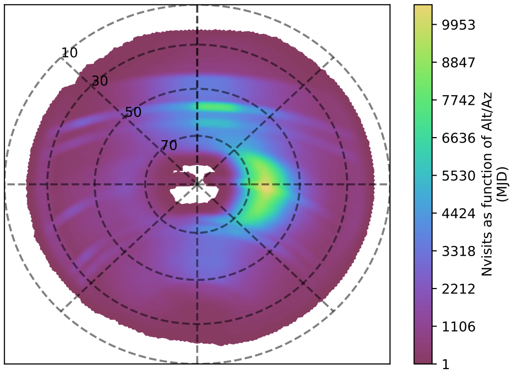
too_ignore_5_1v3.4_10yrs all bands: Nvisits as function of Alt/Az
